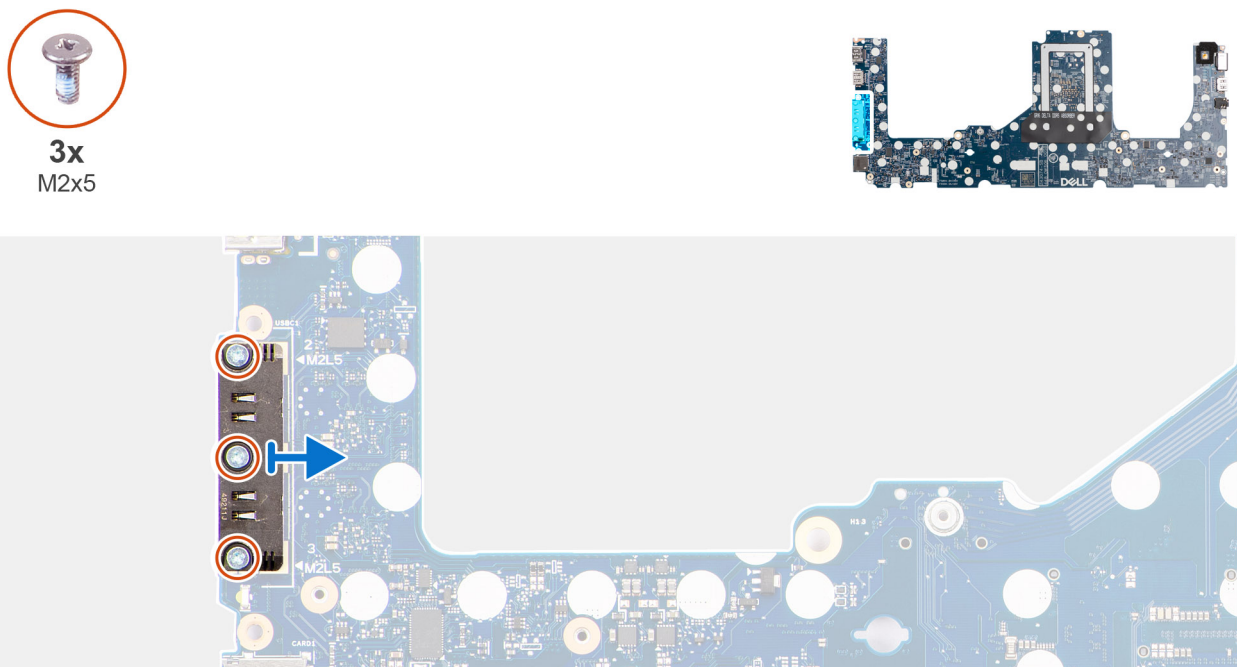
Figure 79. Removing the USB Type-C module
