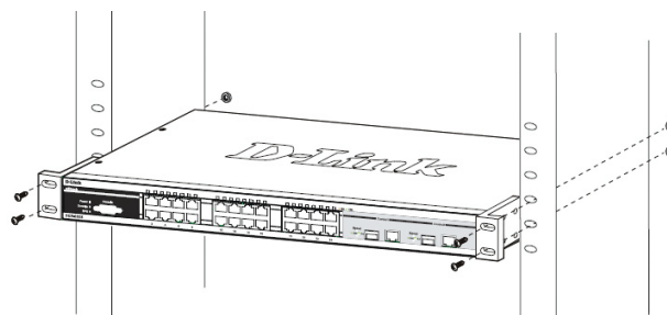
Figure 3. Installing the switch in a standard-sized equipment rack
