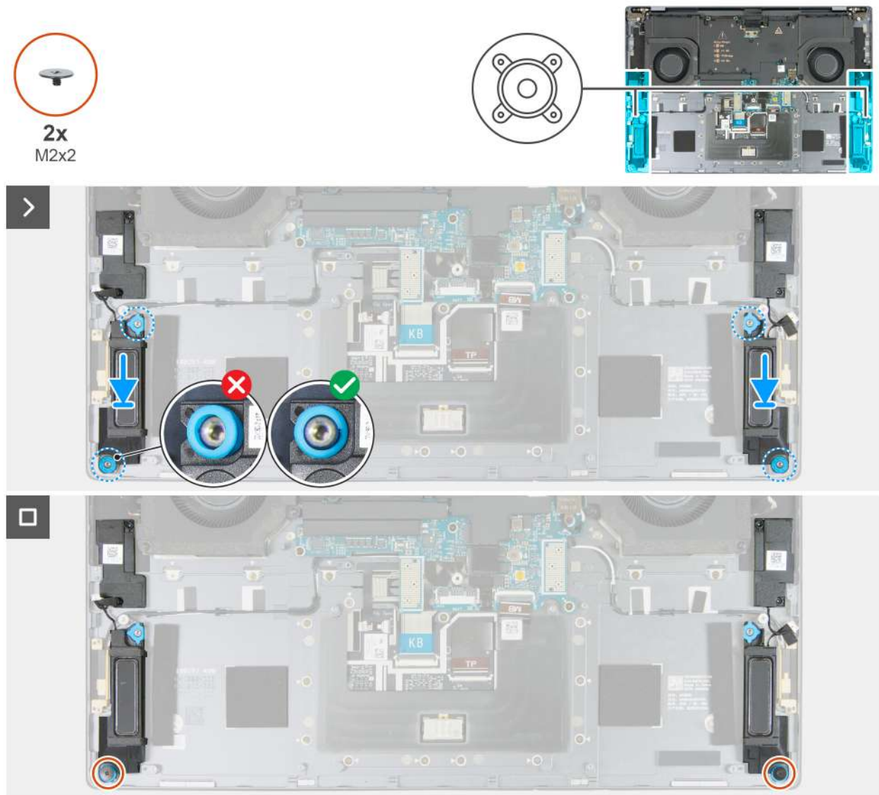
Figure 75. Installing the speakers
