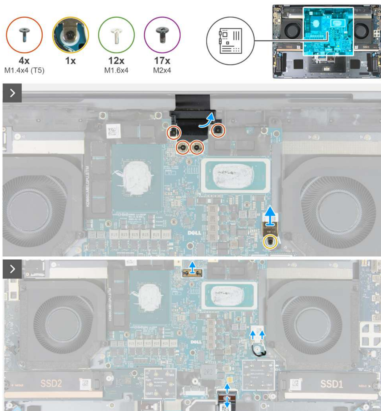
Figure 64. Removing the system board (discrete graphics)
