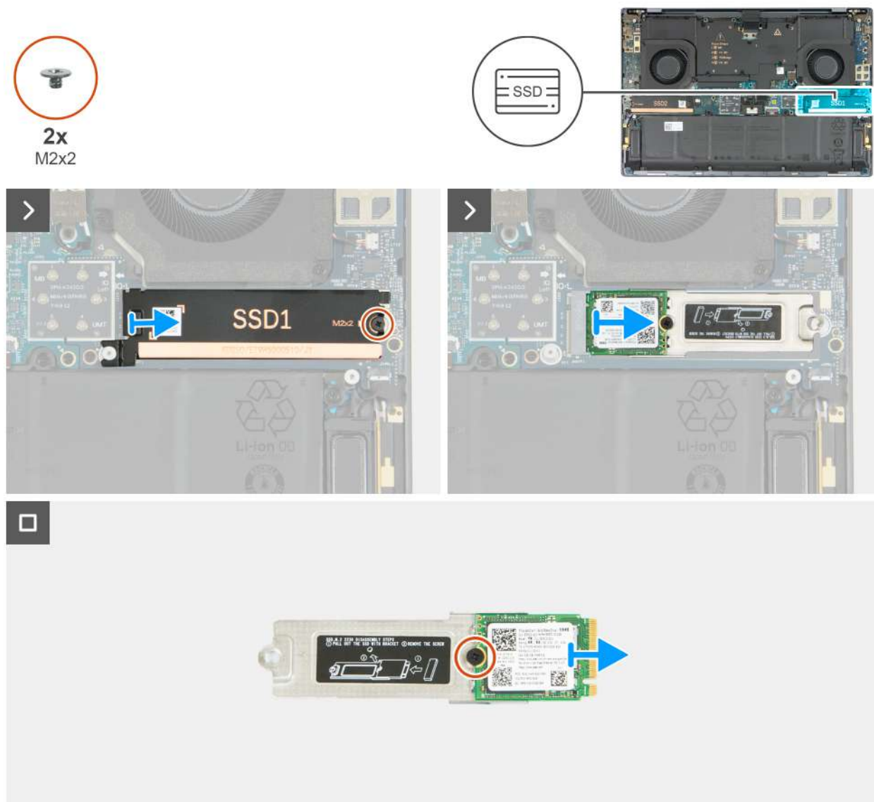
Figure 26. Removing the M.2 2230 solid state drive (SSD1)
