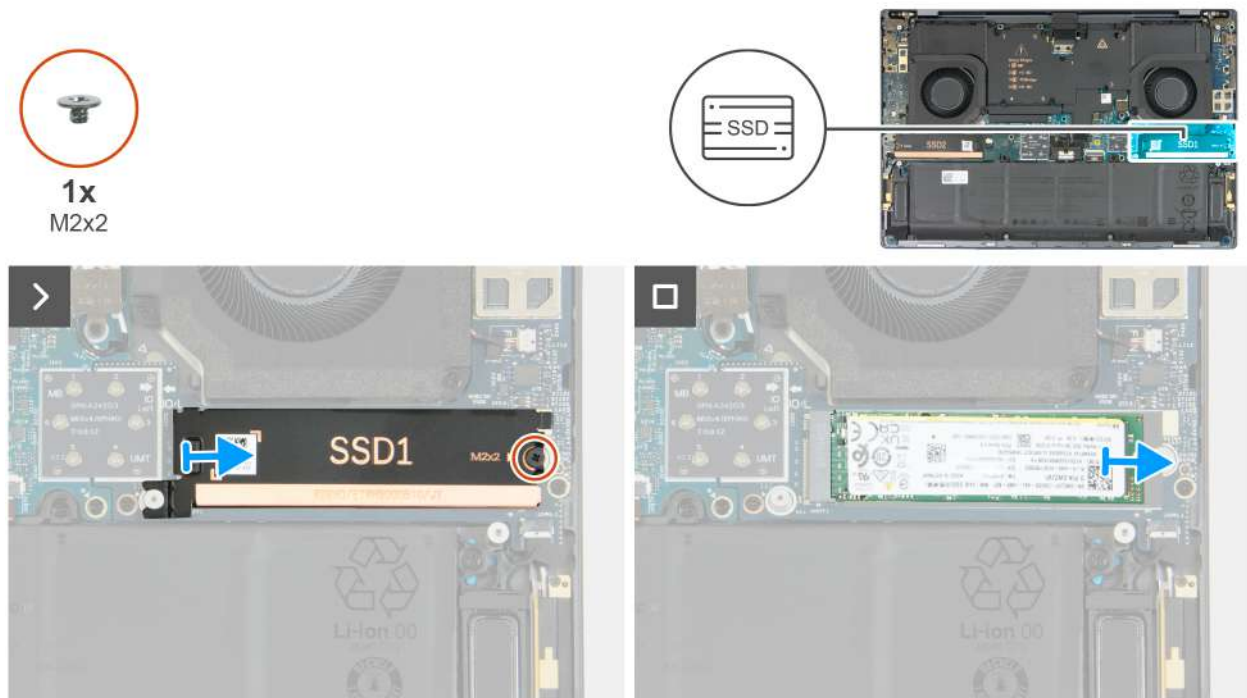
Figure 22. Removing the M.2 2280 solid state drive (SSD1)
