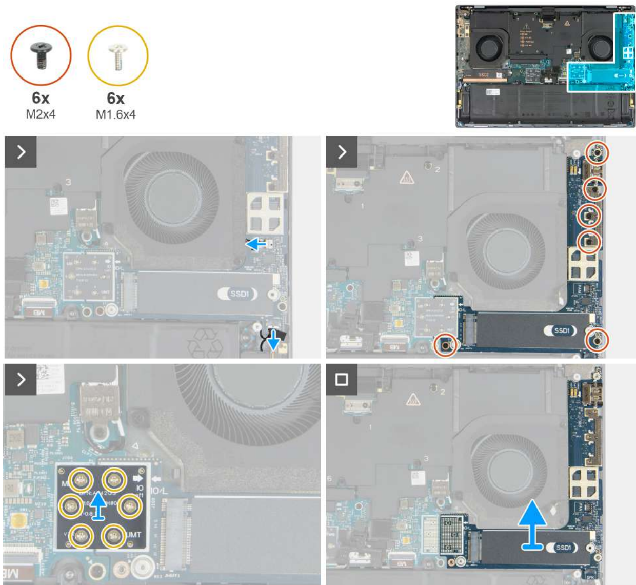
Figure 50. Removing the left I/O-board
